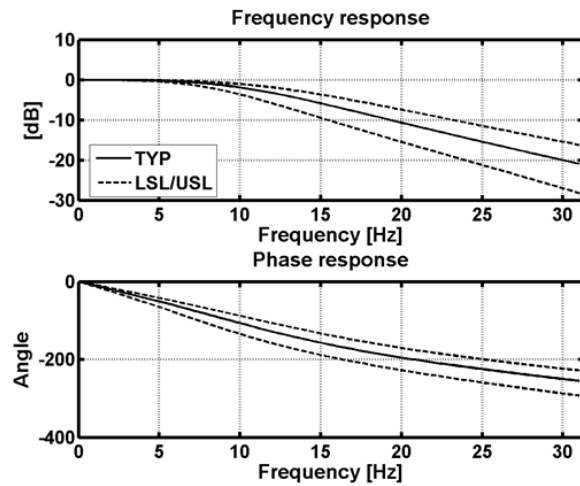
Figure 4 Frequency response of SCA3000-E02 in bypass measurement mode
