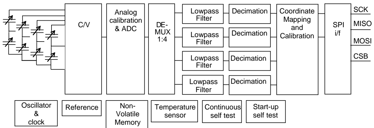
Figure 1. SCA3100-D03 Block diagram
